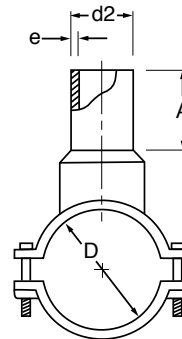
Under Clamp STYLE 3
